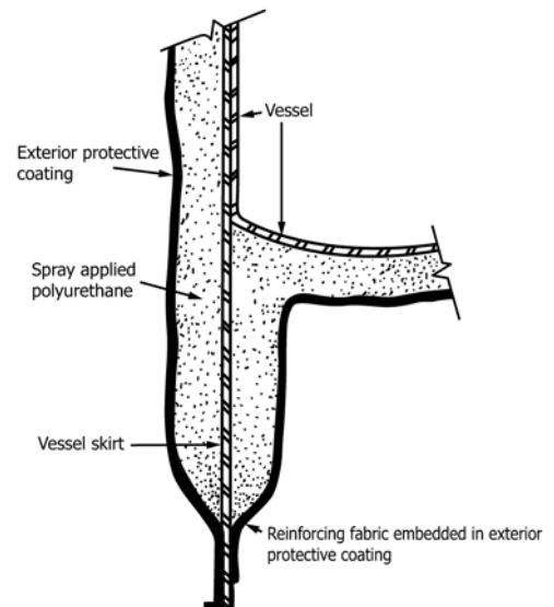
FIG. 6 Insulation of Vessel Skirt
