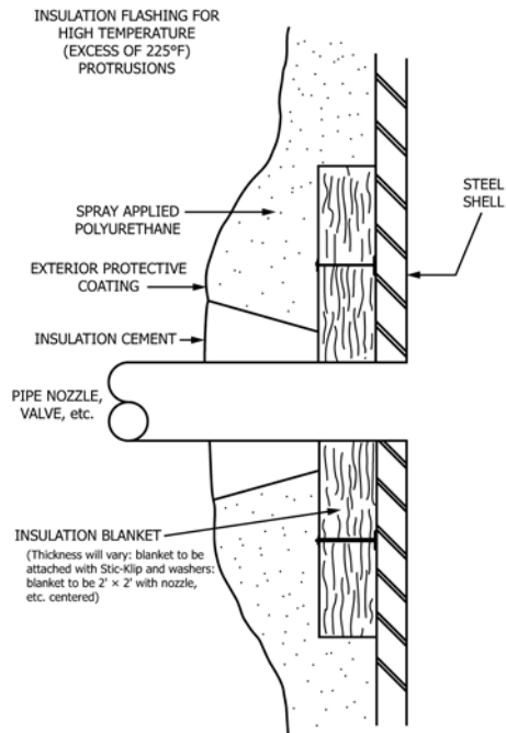
FIG. 8 Insulation Flashing for High-Temperature Protrusions
