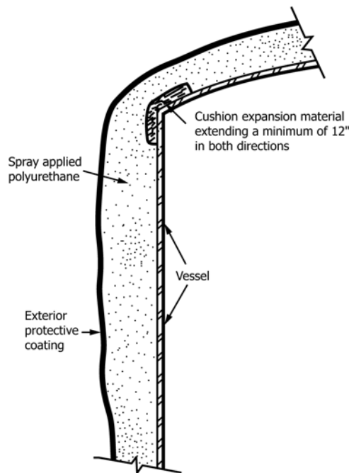
FIG. 3 Typical Insulation Shell and Roof Junction
