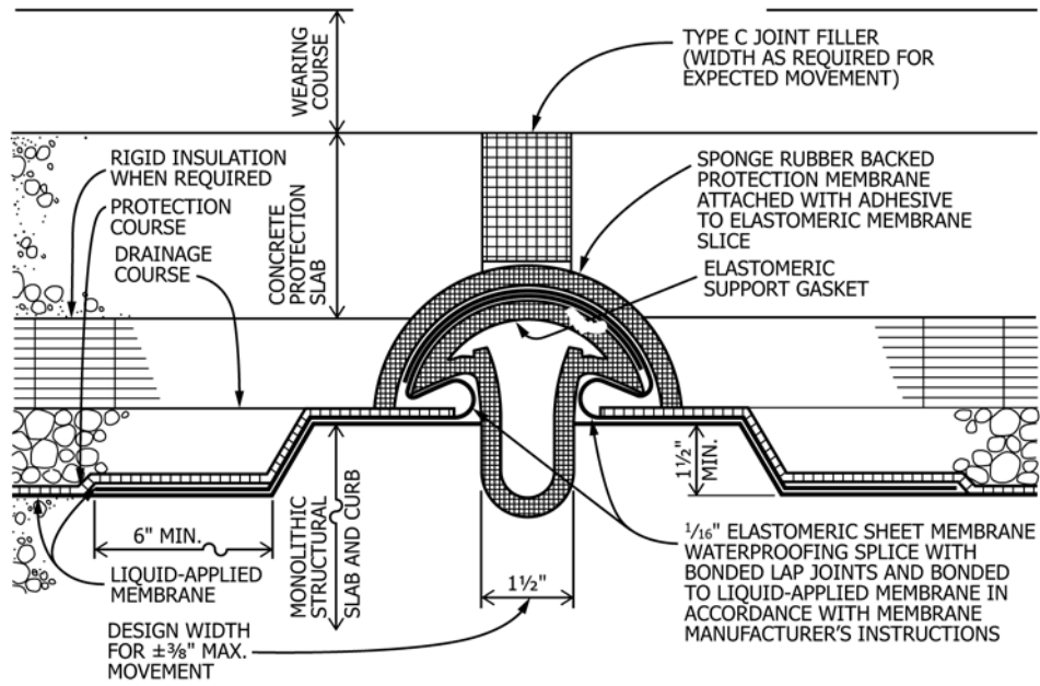
FIG. 11 Water Shed Concept Expansion Joint
