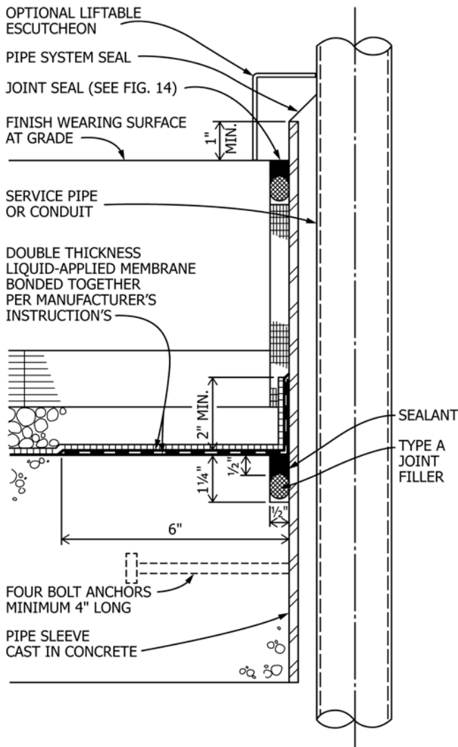
FIG. 7 Termination at Pipe Penetrations (see 7.6.3 and 7.6.1)
