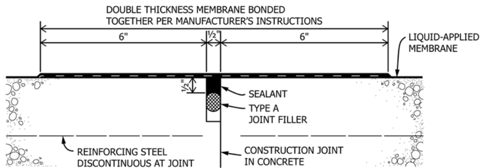
FIG. 9 Treatment of Nonreinforced Butted-Joint in Concrete Slab (see 7.7.3)
