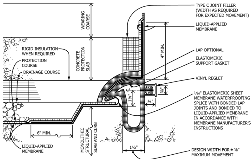
FIG. 12 Water Shed Concept Expansion Joint (see also Fig. 13 for Easier Gasket Installation Detail)
