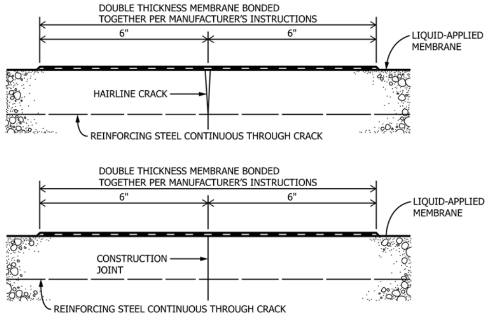
FIG. 8 Treatment of Reinforced Cracks and Joints in Concrete Slab (see 7.7.2)
