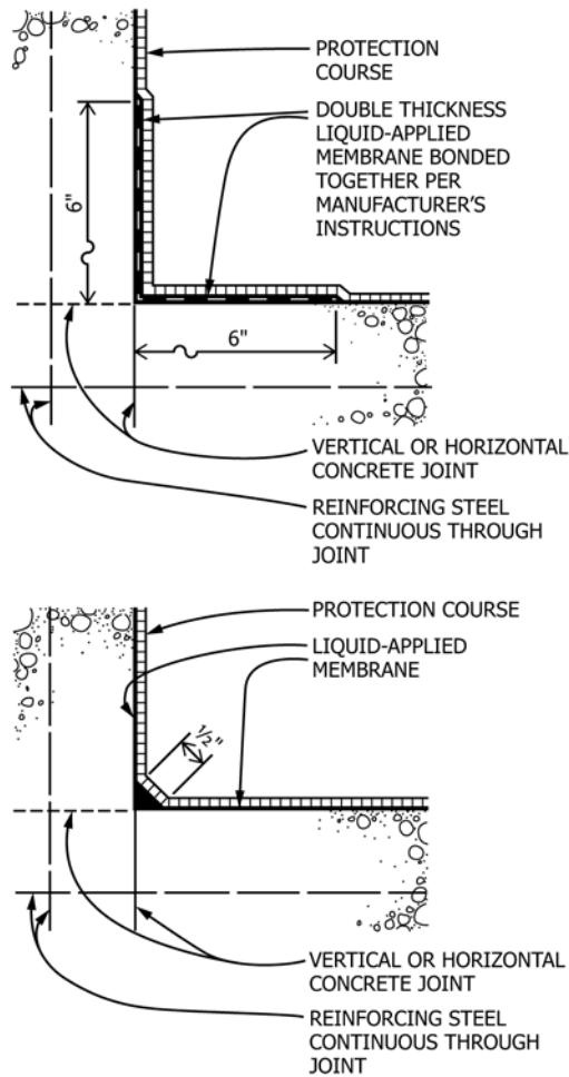
FIG. 5 Turnup Details at Reinforced Joint (see 7.6.3)
