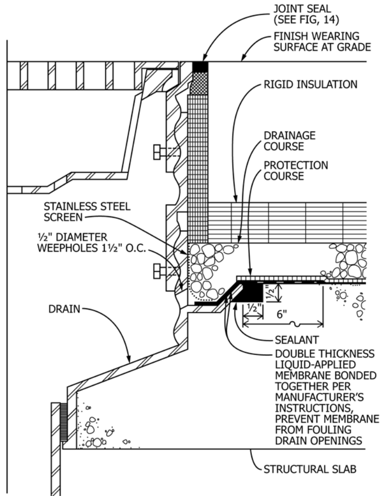
FIG. 6 Termination at Drain
