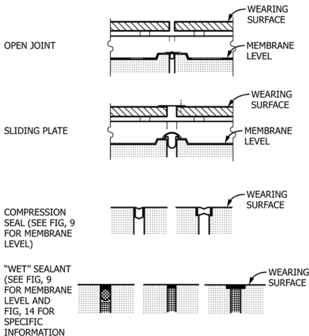
FIG. 14 Schematic Expansion Joint Concepts at Wearing Surface Level
