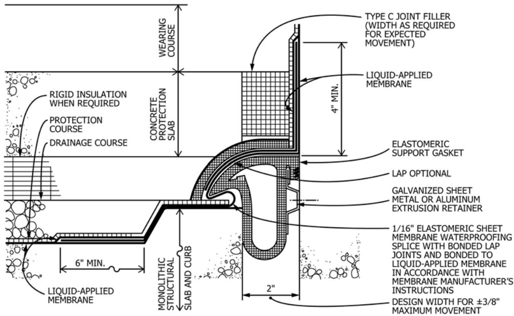
FIG. 13 Water Shed Concept Expansion Joint (see also Fig. 12)
