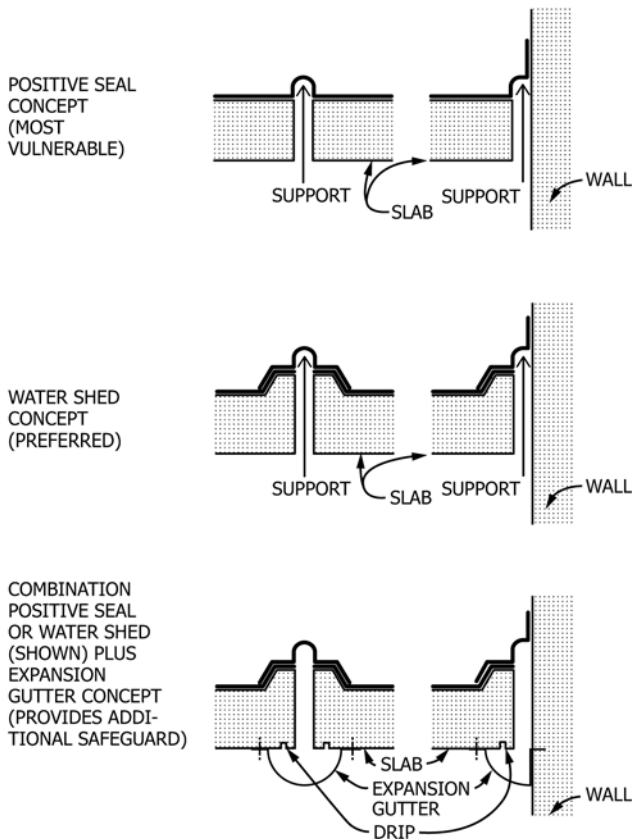
FIG. 10 Schematic Expansion Joint Concepts at Membrane Level
