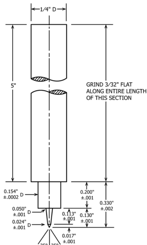
FIG. 2 Venting Tool
