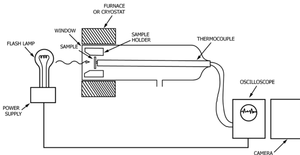
FIG. 3 Schematic Diagram of Apparatus
