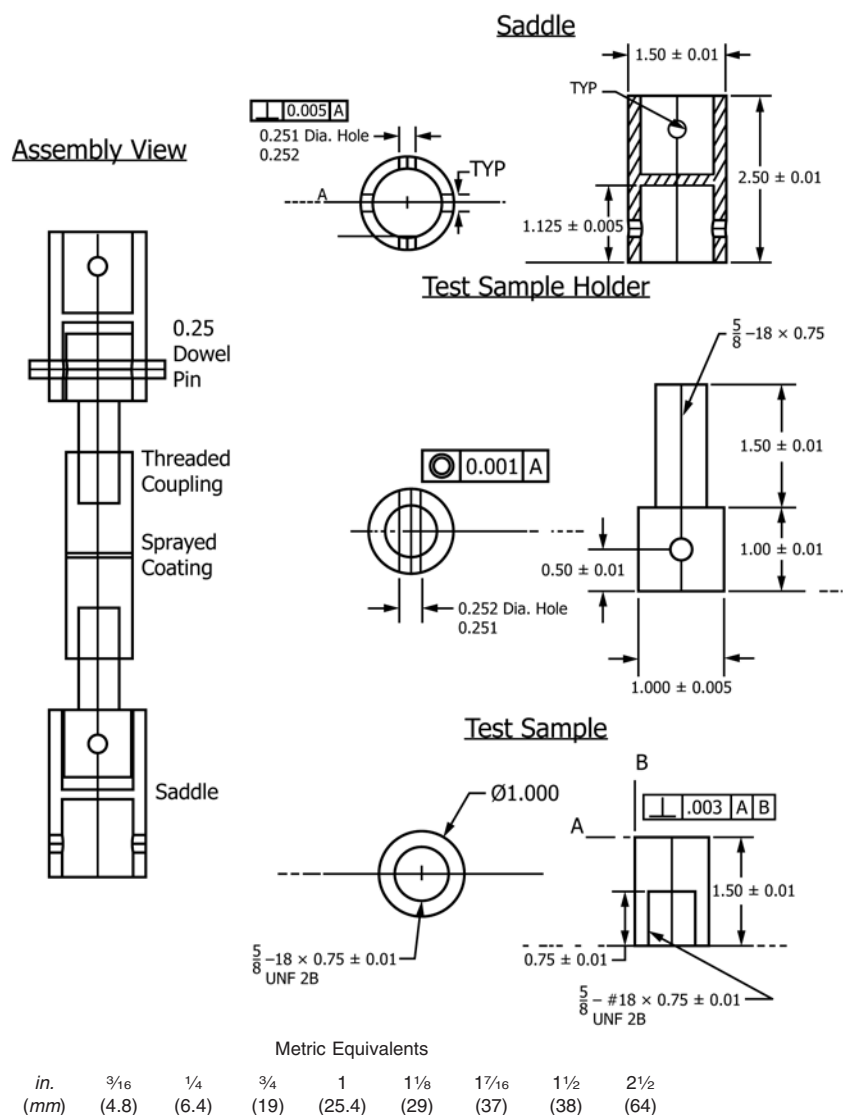
FIG. 1 Self-Aligning Device
