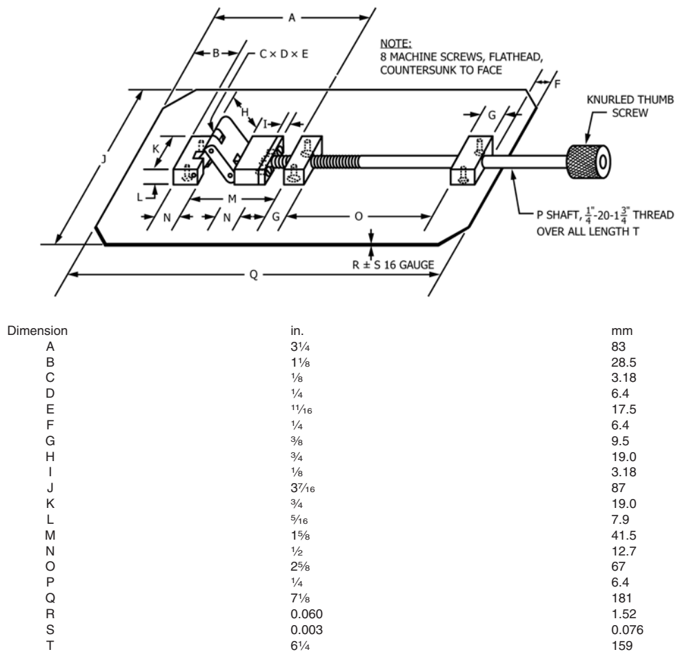
FIG. 7 Stainless Steel Specimen Backup Plate
