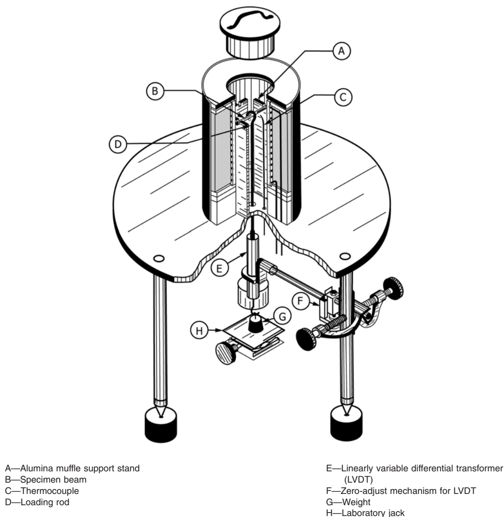
FIG. 1 Cutaway Drawing of Beam-Bending Apparatus
