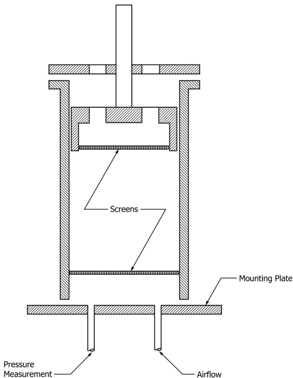
FIG. 2 Specimen Holder
