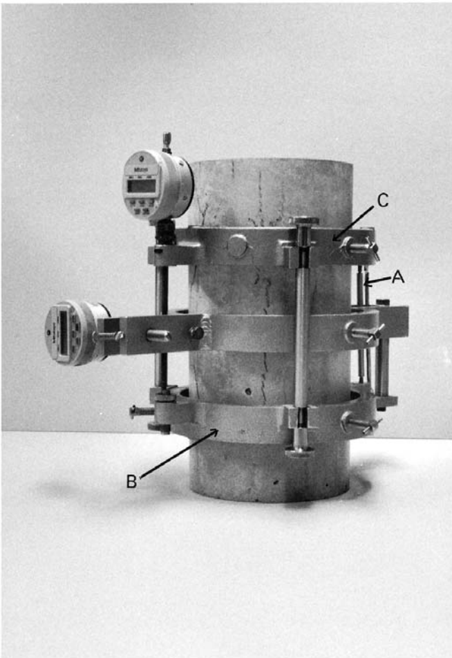
FIG. 1 Suable Compressometer
