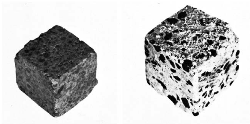
FIG. 2 Rating Basic Brick or Shapes Specimens After Hydration Periods—Rating 1 on Left and Rating 2 on Right
