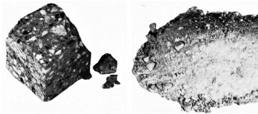
FIG. 3 Rating Basic Brick or Shapes Specimens After Hydration Periods—Rating 3 on Left and Rating 4 on Right
