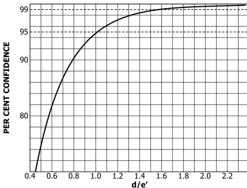
FIG. 1 Variation in Percentage Confidence that a Difference Between Two Determinations is Not Due to Chance Fluctuations with the Ratio d/e' for Samples of Six Specimens
