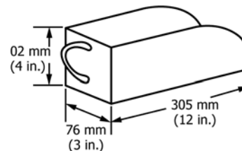
FIG. X2.3 Scoop Sampler
