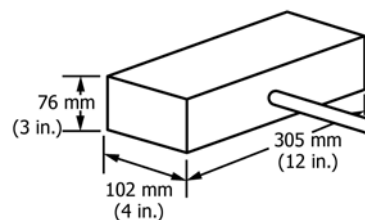
FIG. X2.2 Open Box Sampler
