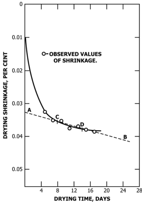
NOTE 1—The interval CD is 6 days on the time scale and % on the shrinkage scale. Point D defines equilibrium shrinkage value. FIG. 3 Graphical Method of Determining Equilibrium Shrinkage
