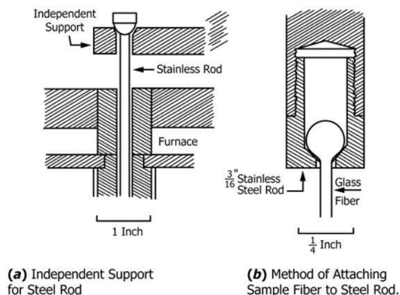
FIG. 4 Apparatus Assembly for Suspension of Sample Fiber Between Metal Rod
