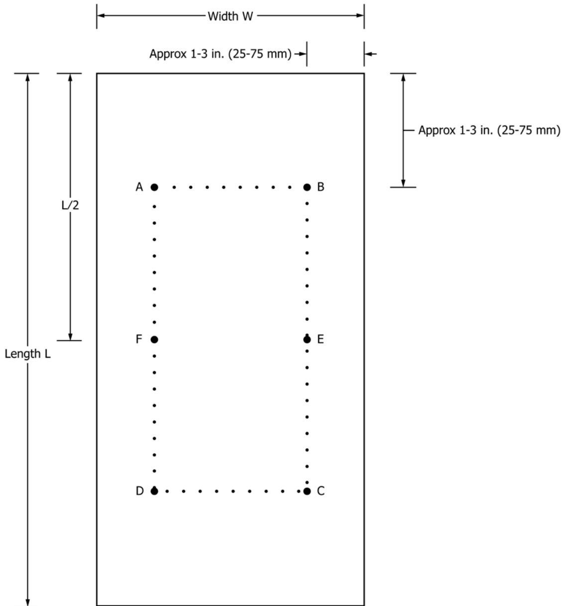
FIG. 1 Specimen Measurement
