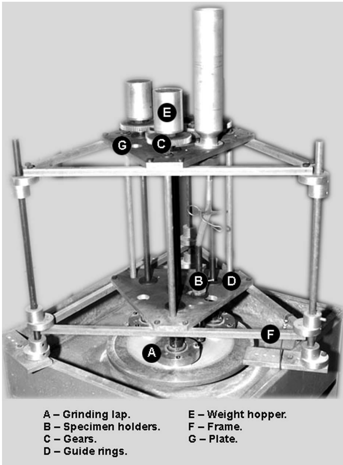
FIG. 1 Apparatus for Abrasion Resistance Test of Stone
