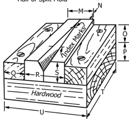
Mold Assembly
