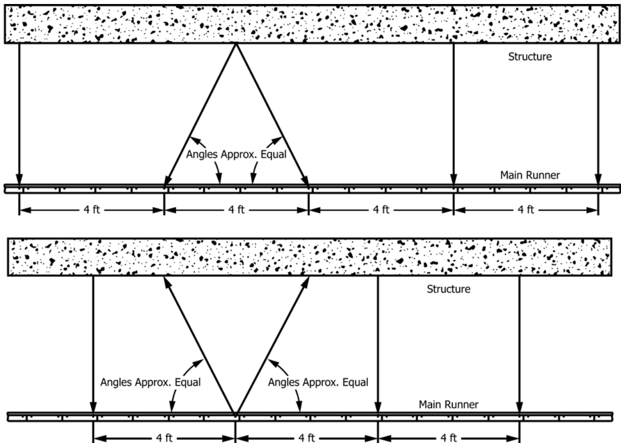
FIG. 1 Allowable Counter Sloping Methods
