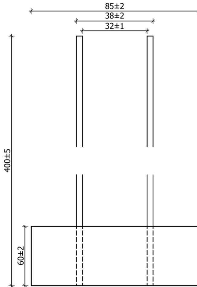
FIG. 6 Suitable Dimensions of the Support Tube That is Used During Filling of the Corrugated Molds
