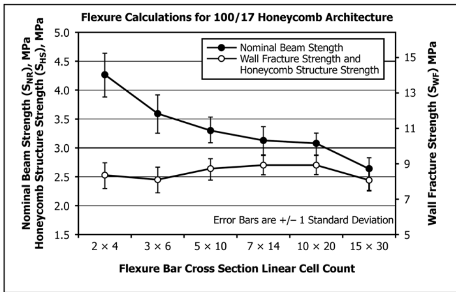
FIG. X1.3 Average S_{NB} , S_{WF} , and S_{HS} Values for Each Size Specimen of the 100/17 Test Set (7)
