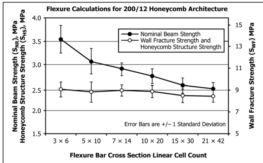
FIG. X1.4 Average S_{NB} , S_{WF} , and S_{HS} Values for Each Size Specimen of the 200/12 Test Set (7)
