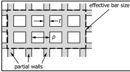
FIG. X1.1 Flexure Bar Cross Section Geometry F (2 x 4) for 100/17 Cell Density (7)
