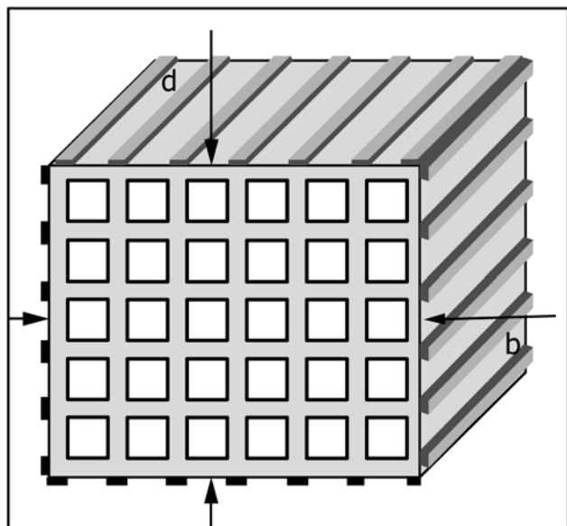
FIG. 7 Thickness and Width Measurement Points Directly on the Specimen Walls (Not Across any Residual Stubs)
