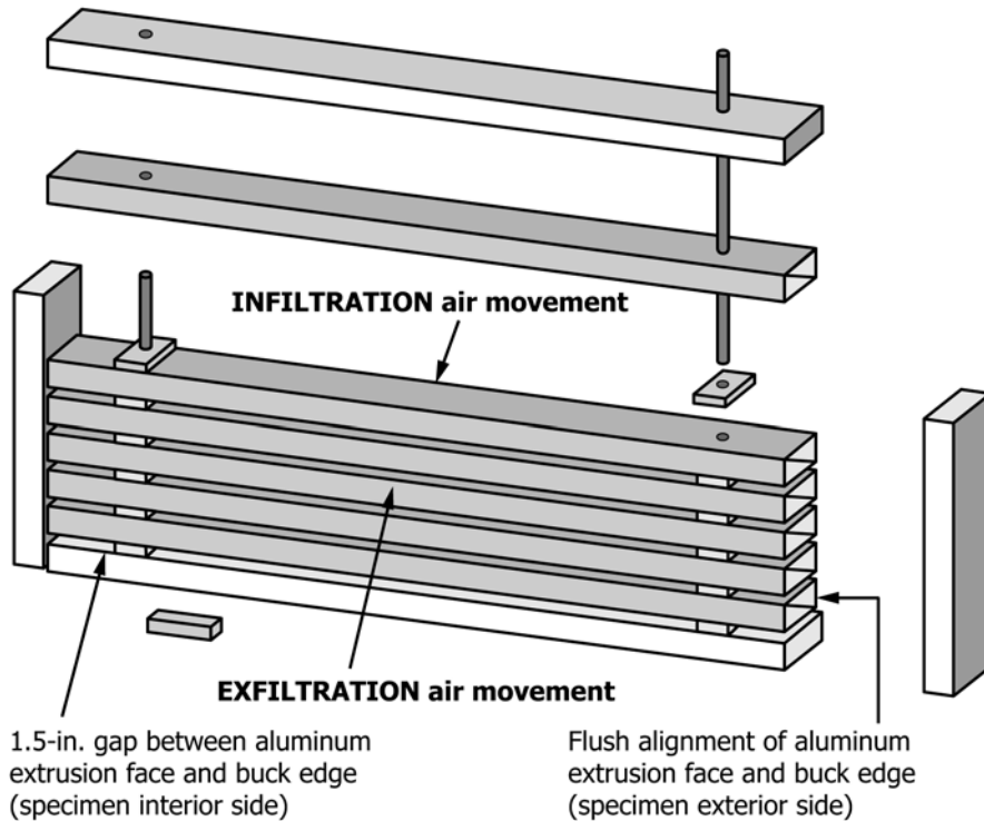
FIG. A1.2 Test Buck – Exploded Assembly
