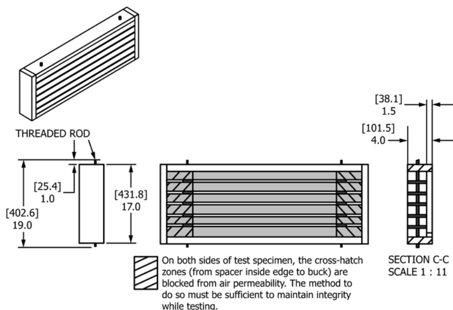
FIG. A1.3 Front View – Assembled Test Buck
