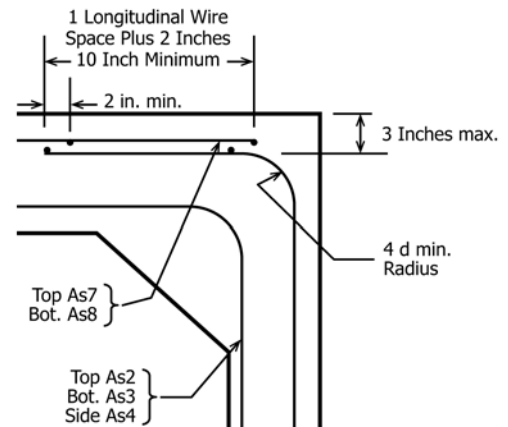
FIG. 6 Detail Option
