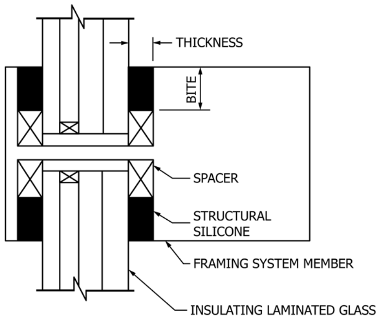
FIG. 6 Generic Missile Impact or Bomb Blast Detail with Insulating Laminated Glass
