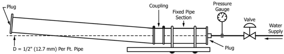
FIG. 1 Deflection Test
