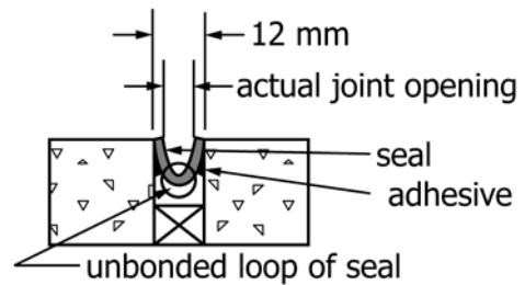
FIG. 3 U-joint Configuration
