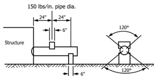
FIG. 1 Shear Test Requirements
