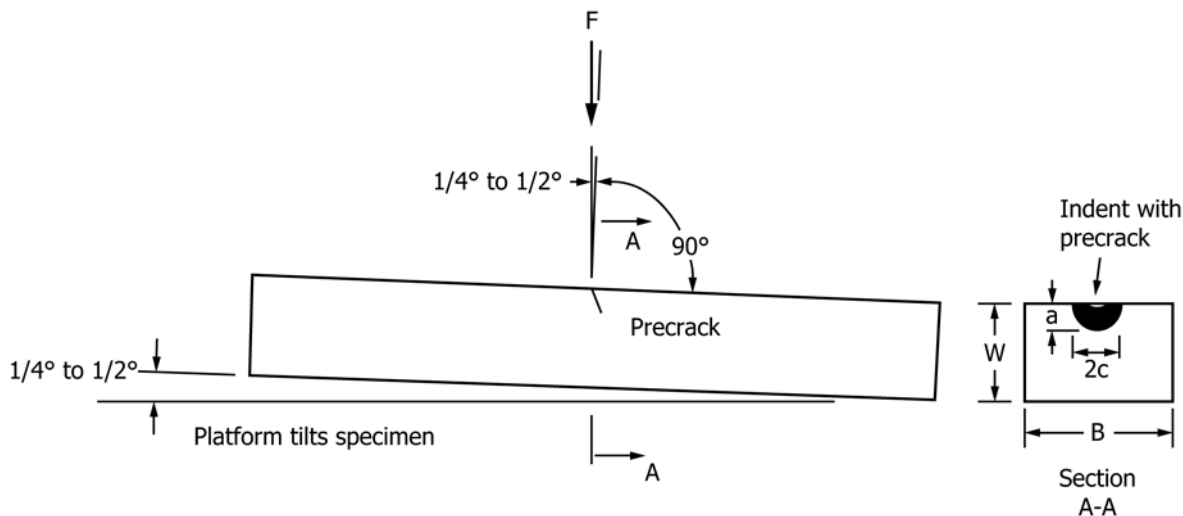
FIG. A3.3 The Test Specimen may be Indented at a \frac{1}{2}^\circ Tilt in Order to Enhance the Chances of Detecting the Precrack on the Fractographic Surface During Subsequent Fracture Analysis. The indentation may be introduced in either the narrow 3-mm face or the wide 4-mm face.
