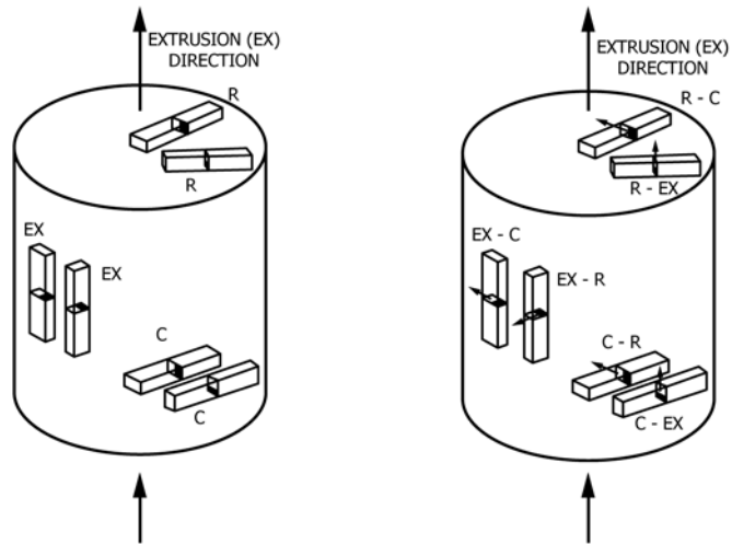
FIG. X5.1 Crack Plane Orientation Code for Hot-Pressed Products
