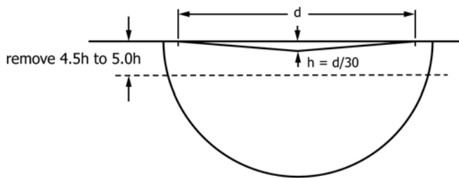
FIG. A3.5 The Precrack Extends Below the Knoop Hardness Impression, which has Depth, h
