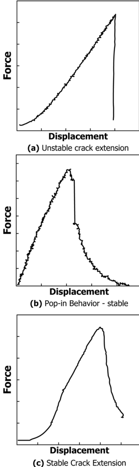
FIG. A2.6 Force Displacement Diagrams from Precracked Beam Tests
