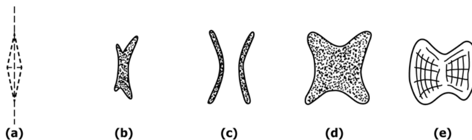
FIG. A3.6 Remnants of Lateral Cracks
