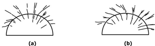
FIG. X1.6 Fine Hackle Lines may Change Direction at the Pre-crack Boundary
