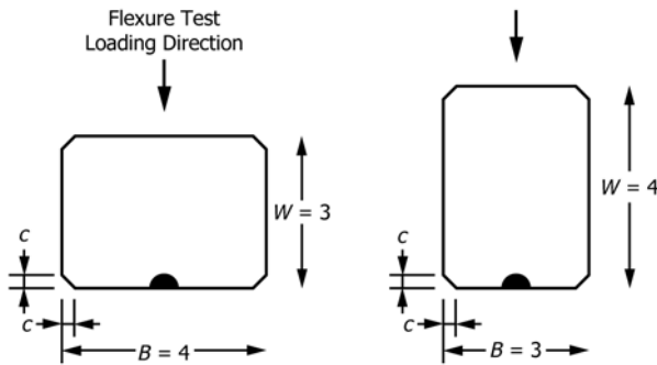
FIG. X4.1 sc Test Specimen Cross Section
