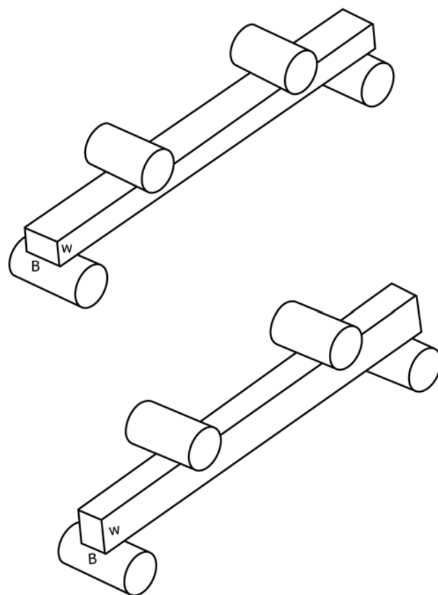
FIG. A3.7 The Flexure Specimen Can be Tested with Either the Wide or Narrow Face on the Flexure Rollers
