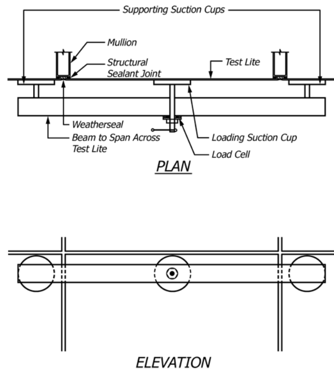
FIG. 1 Schematic of Field Loading Device
