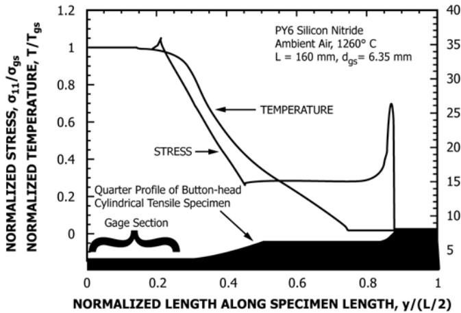
FIG. 9 Example of Superposed Stress and Temperature Results from Finite Element Analyses of a Monolithic Silicon Nitride, Button-Head Tensile Test Specimen with Water-Cooled Grips and Resistance-Heated Furnace Heating Only the Center 50 mm of the Test Specimen
