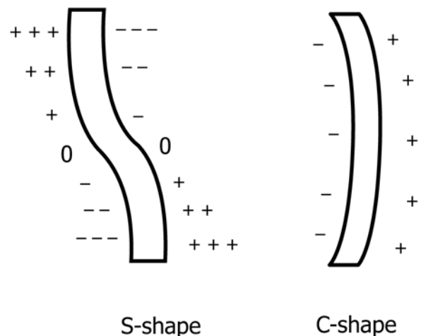
FIG. X1.2 S-Shape and C-Shape Bending of Tensile Test Specimens
