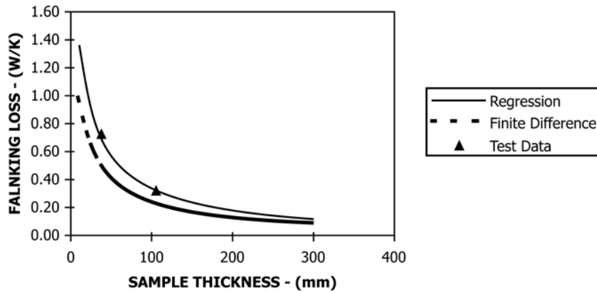
FIG. A7.3 Relationship of Flanking Loss to Specimen Thickness (Estimated vs. Tested)
