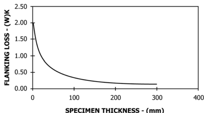
FIG. A7.1 Relationship of Flanking Loss to Specimen Thickness (Estimated with Modeling)
