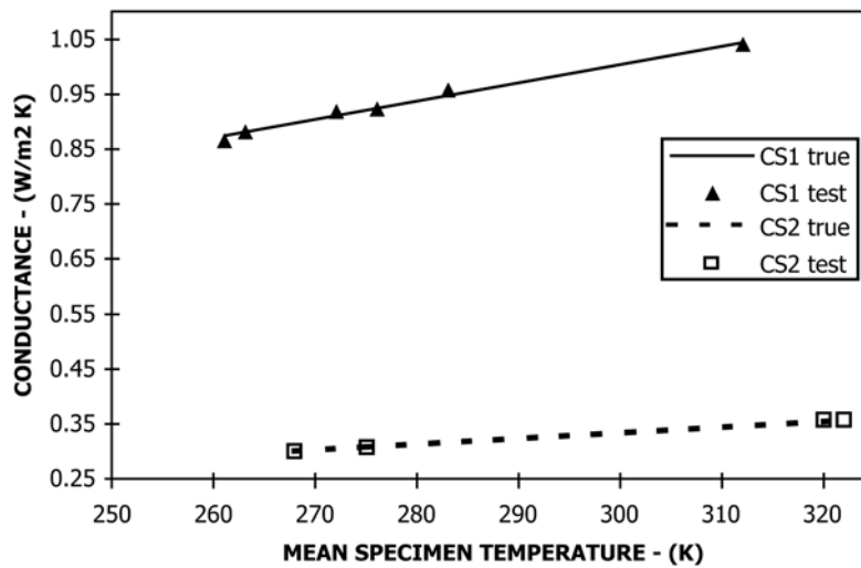
FIG. A7.4 Relationship of Conductance to Mean Specimen Temperature
