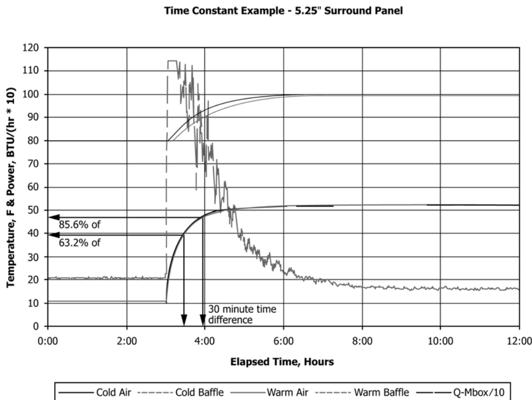
FIG. A10.1 Example Data Time Constant Determination
