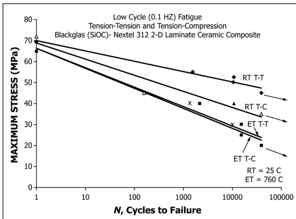
FIG. 2 Fatigue (Tension-Tension and Tension-Compression) Behavior of Blackglas (SiOC)-Nextel 312 Ceramic Composite at Room Temperature and 760 °C
