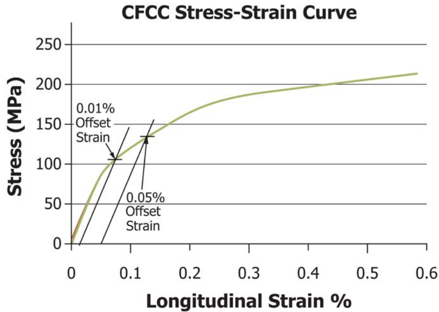
FIG. 10 CFCC Stress-Strain Curve with Two Offset Strain Values
