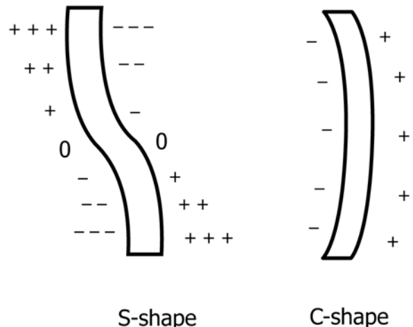
FIG. X1.2 S-Shape and C-Shape Bending of Compressive Test Specimen
