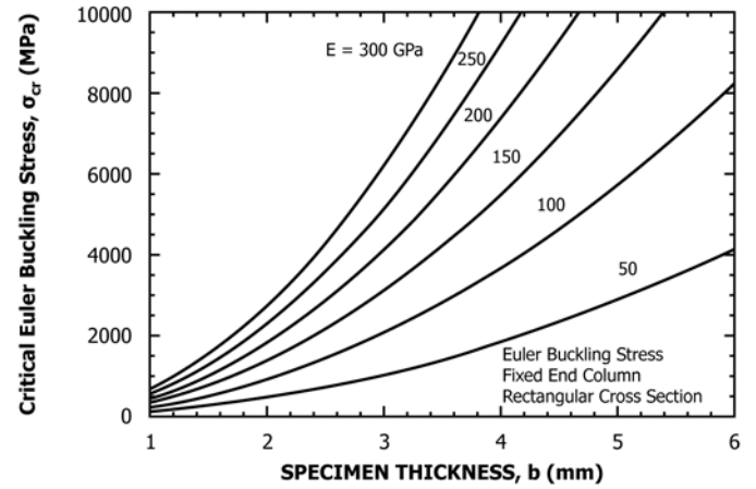
FIG. X2.1 Critical Euler Buckling Stress for Fixed-End Column With Rectangular Cross Section of Width 10 mm
