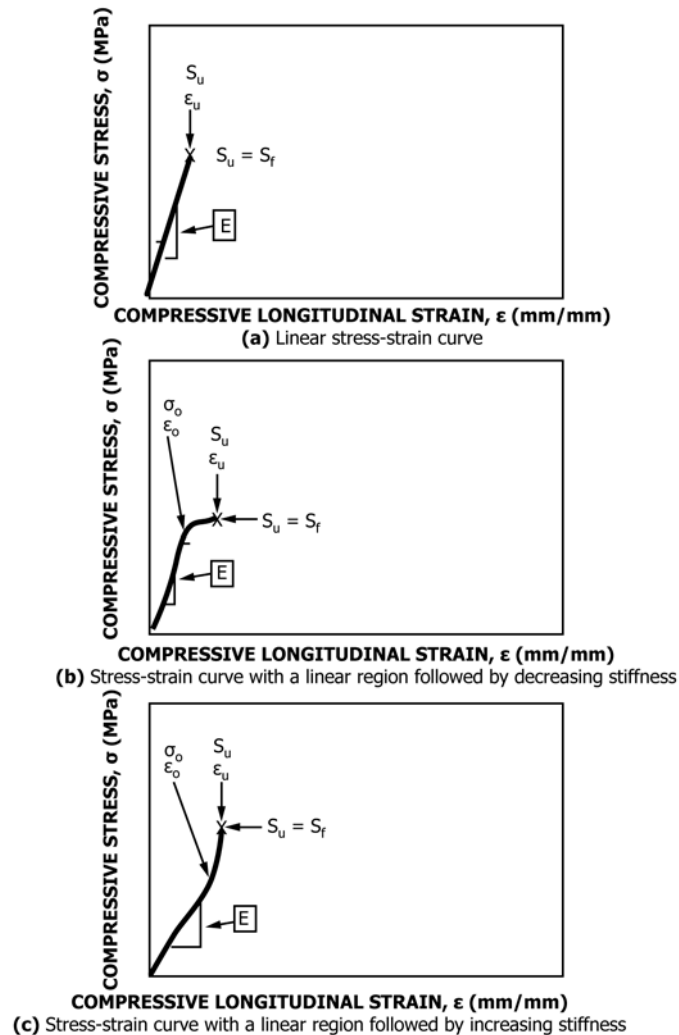
FIG. 8 Schematic Diagrams of Compressive Stress-Strain Curves for CFCCs
