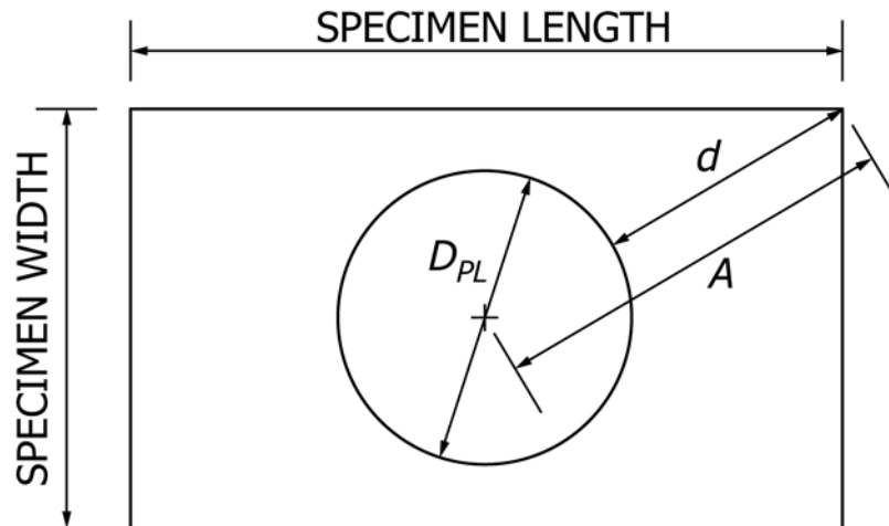
FIG. A1.3 Distance from Platen to Furthest Corner of Test Specimen
