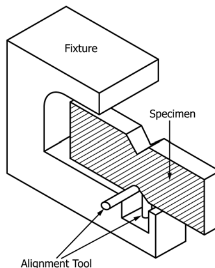
FIG. 8 Specimen Placement in Test Fixture
