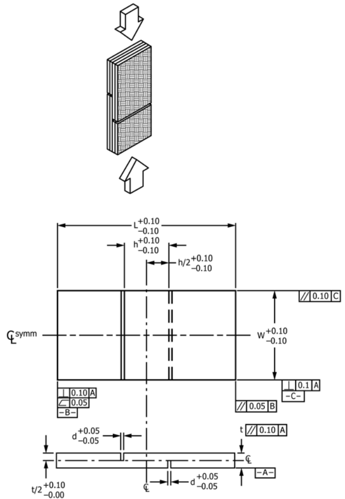
FIG. 2 Schematic of Double-Notched Compression Test Specimen
