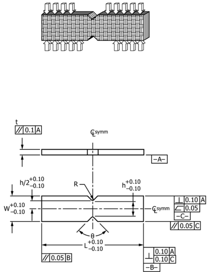
FIG. 5 Schematic of the Iosipescu Specimen
