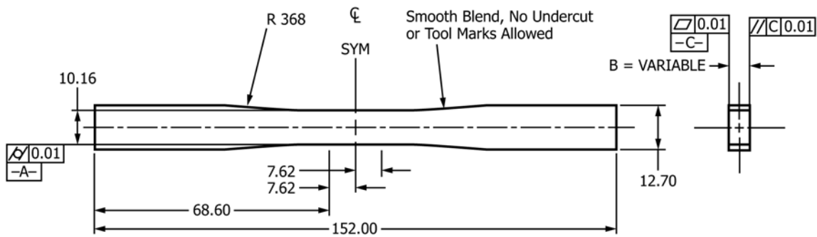
FIG. X2.2 Example of a Contoured, Edge-Loaded Test Specimen Geometry (3)
