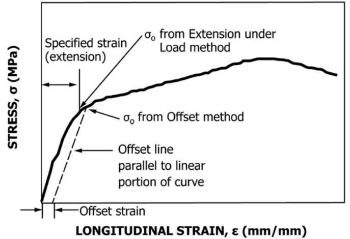
FIG. 10 Schematic Diagram of Methods for Determining Proportional Limit Stress
