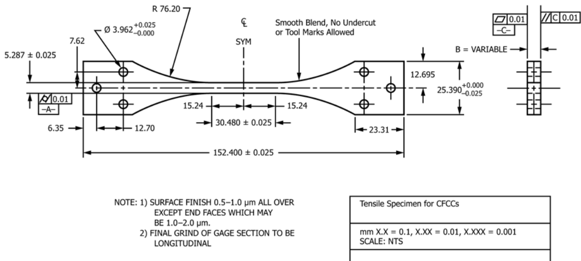
FIG. X2.6 Example of a Contoured, Pin/Face-Loaded Test Specimen Geometry (4)
