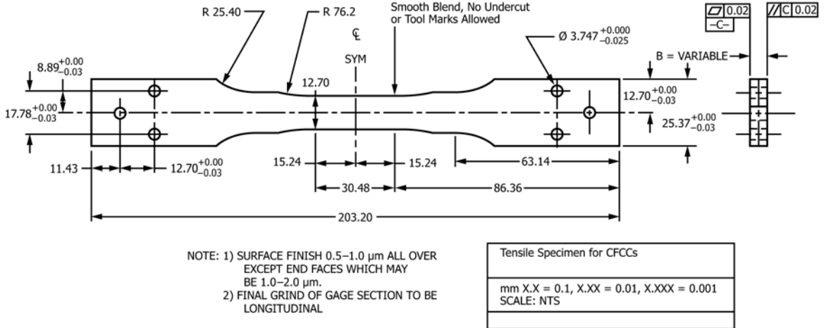
FIG. X2.8 Example of a Contoured, Pin/Face-Loaded Test Specimen Geometry (5)
