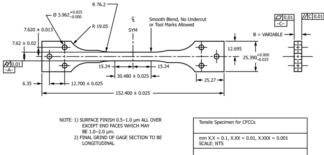
FIG. X2.7 Example of a Contoured, Pin/Face-Loaded Test Specimen Geometry (4)
