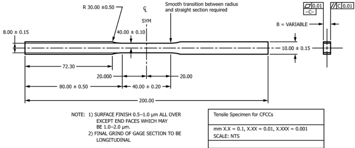
FIG. X2.4 Example of a Contoured, Face-Loaded Test Specimen Geometry
