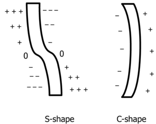
FIG. X1.2 S-Shape and C-Shape Bending of Tensile Specimen
