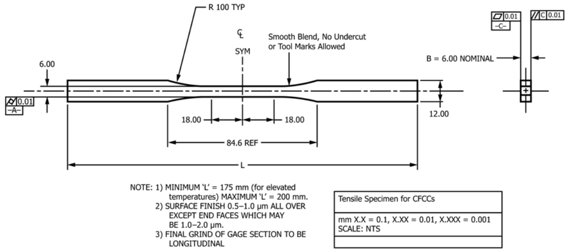
FIG. X2.5 Example of a Contoured, Face-Loaded Test Specimen Geometry
