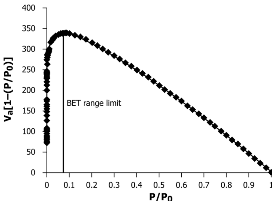
FIG. A2.1 Plot Used to Determine the Upper Limit (Graph Maximum) for the BET Range ( \text{N}_2/77.35\text{K} Adsorption) in a Microporous Silicon Carbide Derived Carbon
