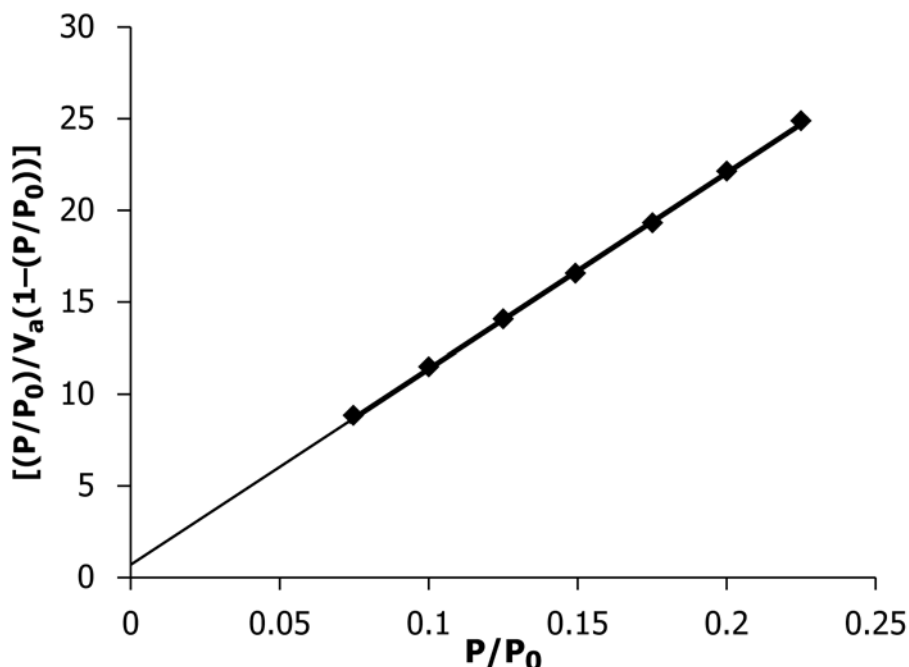
FIG. A1.1 BET Plot for N 2 (77.35K) on a Mesoporous SiO 2 Glass
