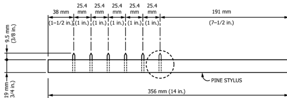
FIG. A1.3 Side View of Puncture Stylus
