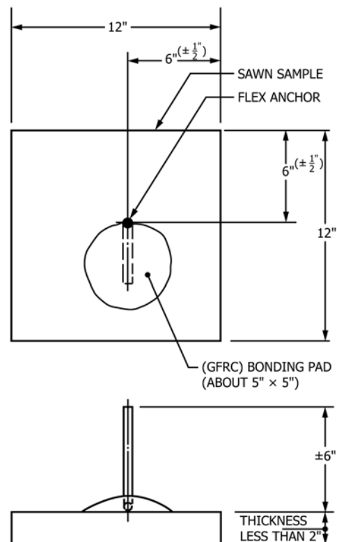
FIG. 4 Test Specimen
