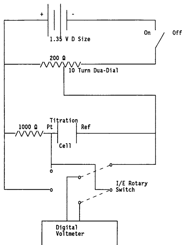
FIG. 1 Amperometric Detector Circuit
