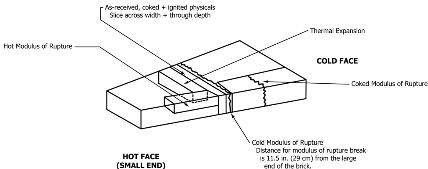
FIG. 1 Location of Test Specimens from Magnesia-Carbon, Impregnated Burned Brick
