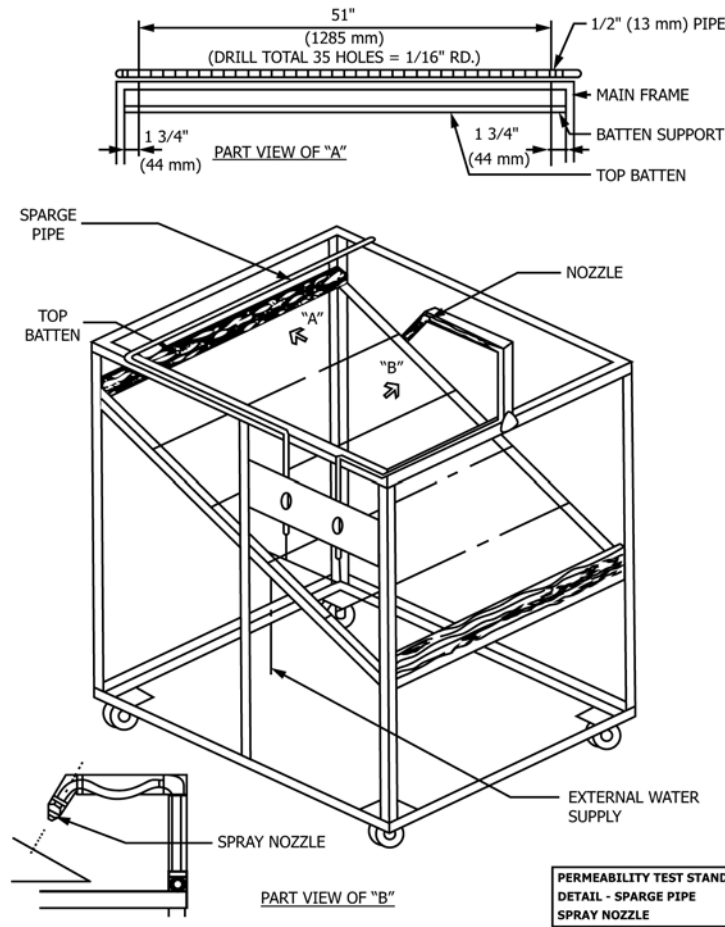
FIG. 2 Deluge Pipe
