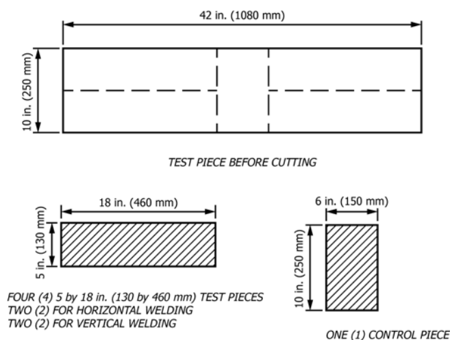
FIG. 1 Test Pieces
