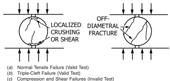
FIG. 2 Failure Modes
