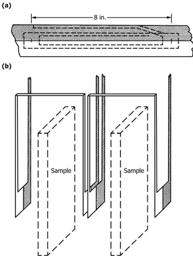
FIG. A1.2 Details of Differential Thermocouple Configuration
