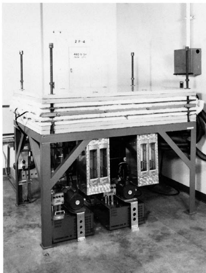
FIG. A2.1 Assembled Metal-Screen Heater Apparatus Without Perimeter Insulation
