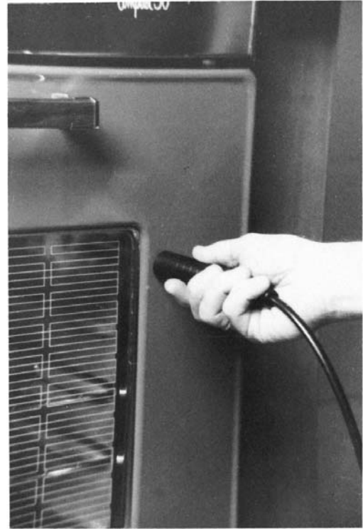
FIG. 4 Applying the Thermesthesiometer to a Vertical Surface
