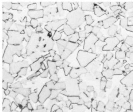
FIG. 3 Apparent Grain Size of Tungsten Carbide plus 18 % Cobalt (1500×)
