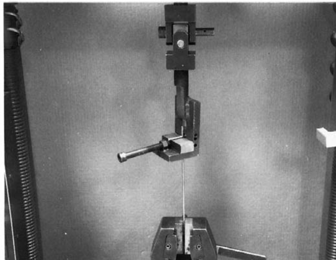
FIG. X1.2 Test Set-up for Ladder-Type Joint Reinforcement (b)
