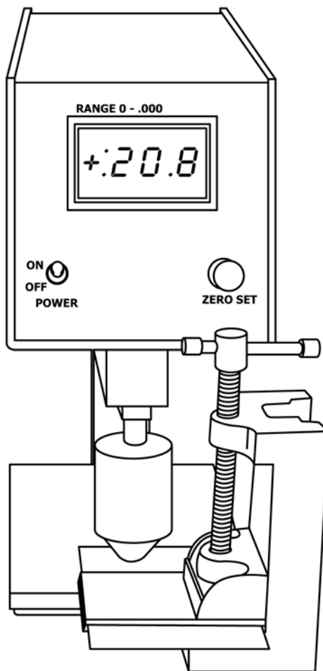
FIG. X1.2 Holding Fixture in Position for Thickness Measurement
