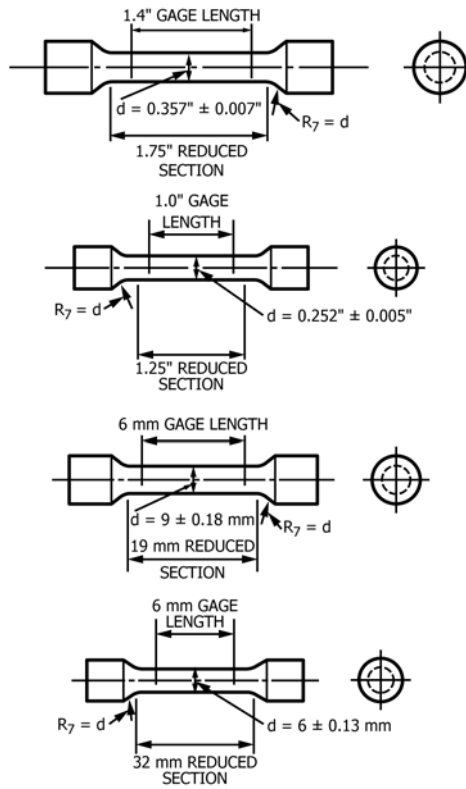
FIG. 6 Examples of Small-Size Specimens Proportional to Standard 1/2-in. [13-mm] Round Specimen
