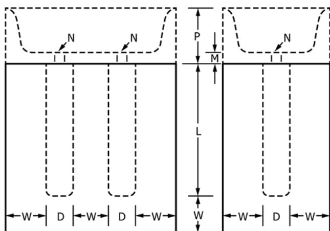
FIG. 4 Design and Dimensions for Mold for Separately Cast Cylindrical Test Bars
